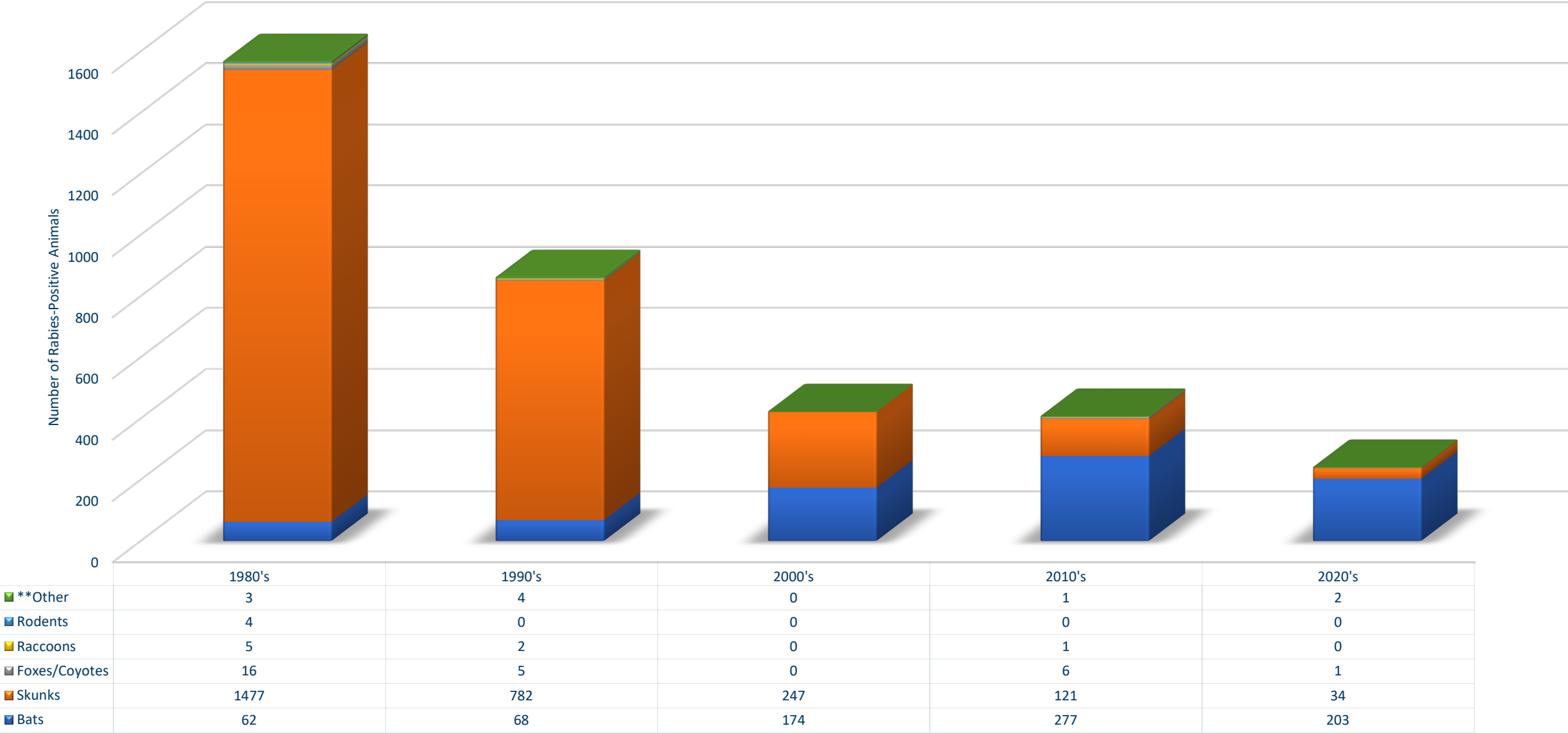
Rabies in Minnesota Wild Species (1975-Present*)
